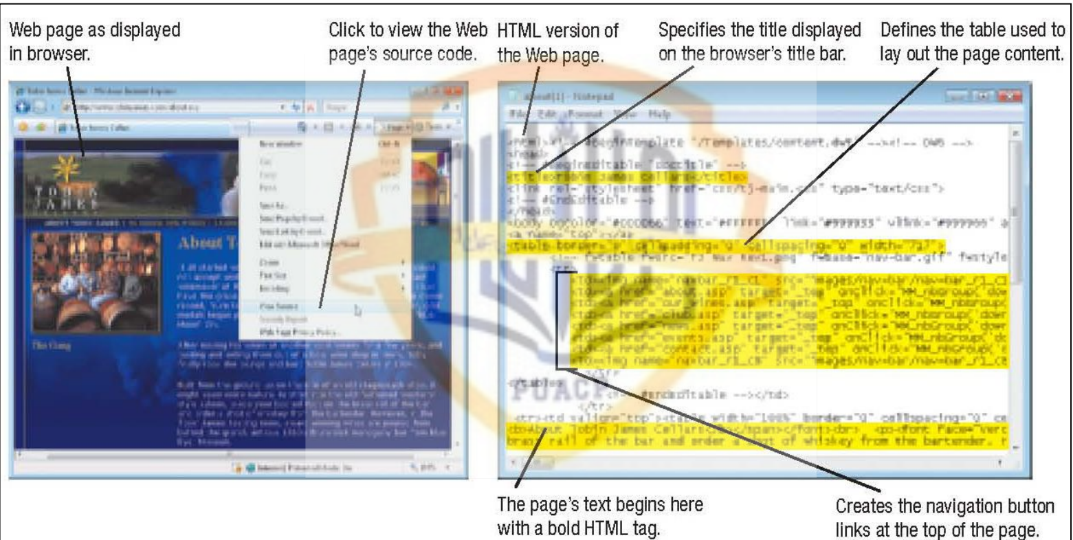
FIGURE 10-18 An HTML Web page and its corresponding source code.
